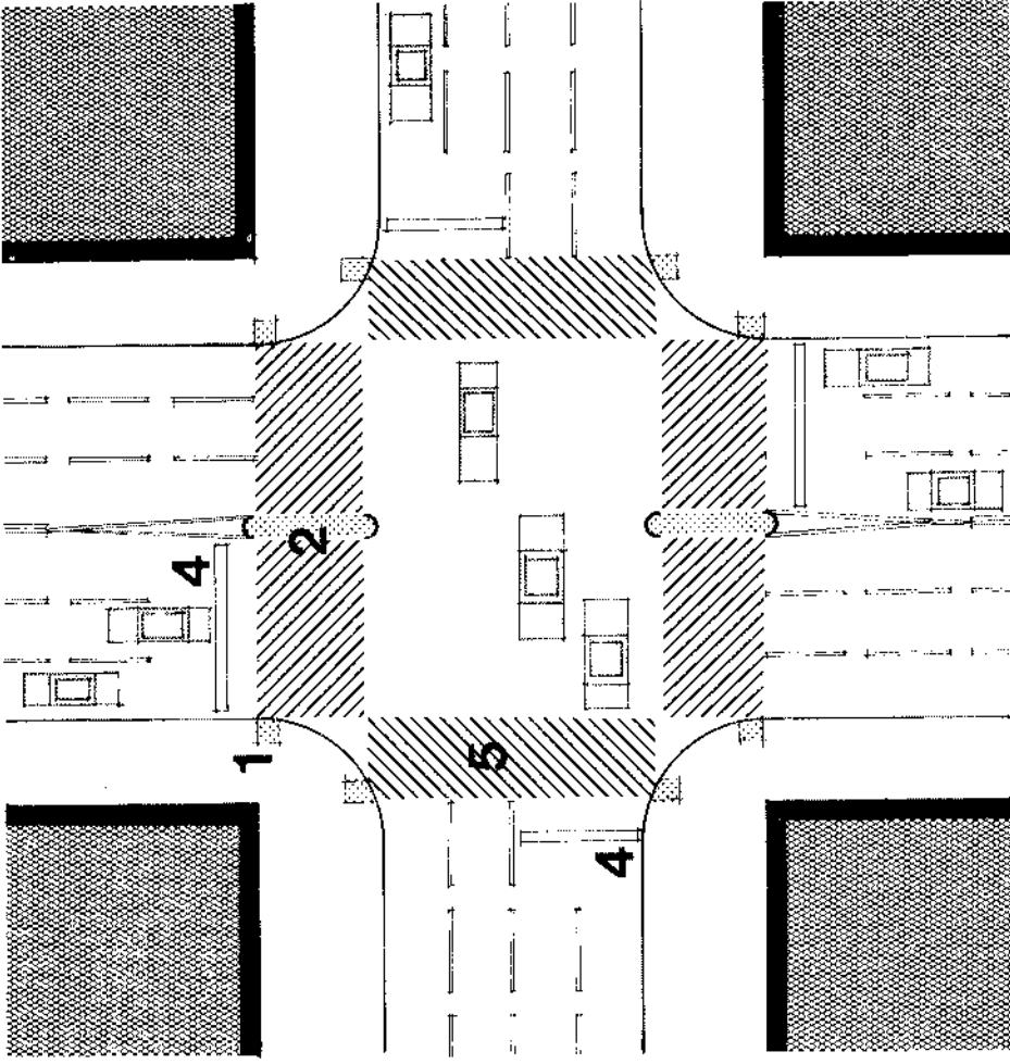
Island occurring in crosswalks at signalized intersection
