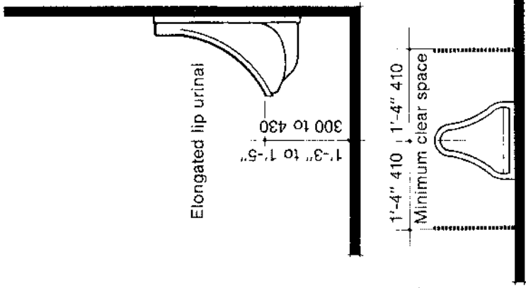
Figure 8.1.12 Wall mounted urinal
