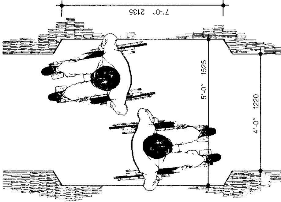
Figure 3.2.1 Minimum dimensions of passing areas in walks less than 5'-0" wide
