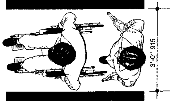
Figure 2.3.4 A Minimum corridor width. Does not allow passing.
