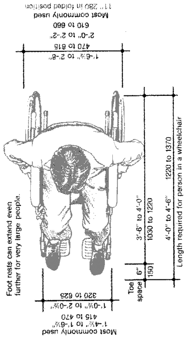
Figure 2.3.1 Dimensions of wheelchairs
