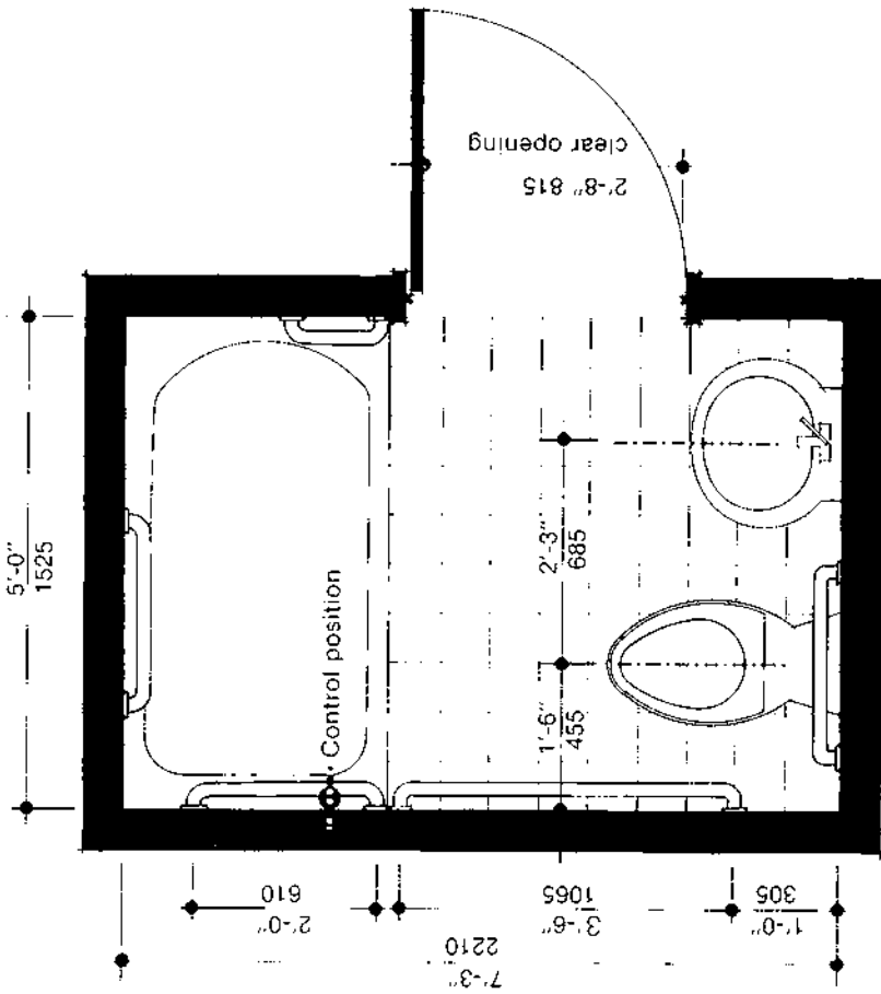
Figure 16.2.4 Example of minimum requirements for a fully accessible bathroom.
