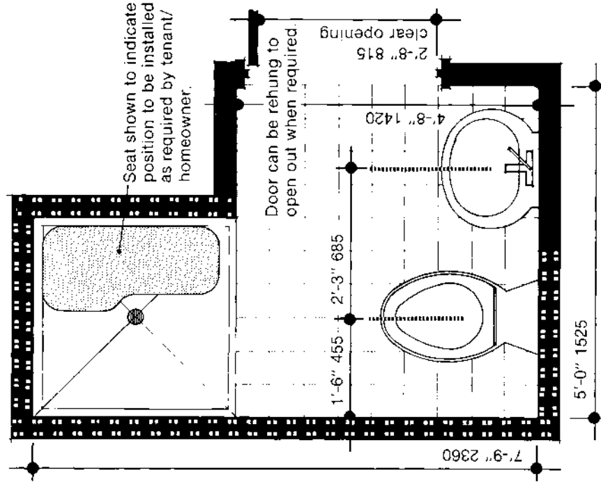
Dotted line indicates lengths of wall to have reinforcement to receive grab bars or supports to be supplied by owner/tenant.
