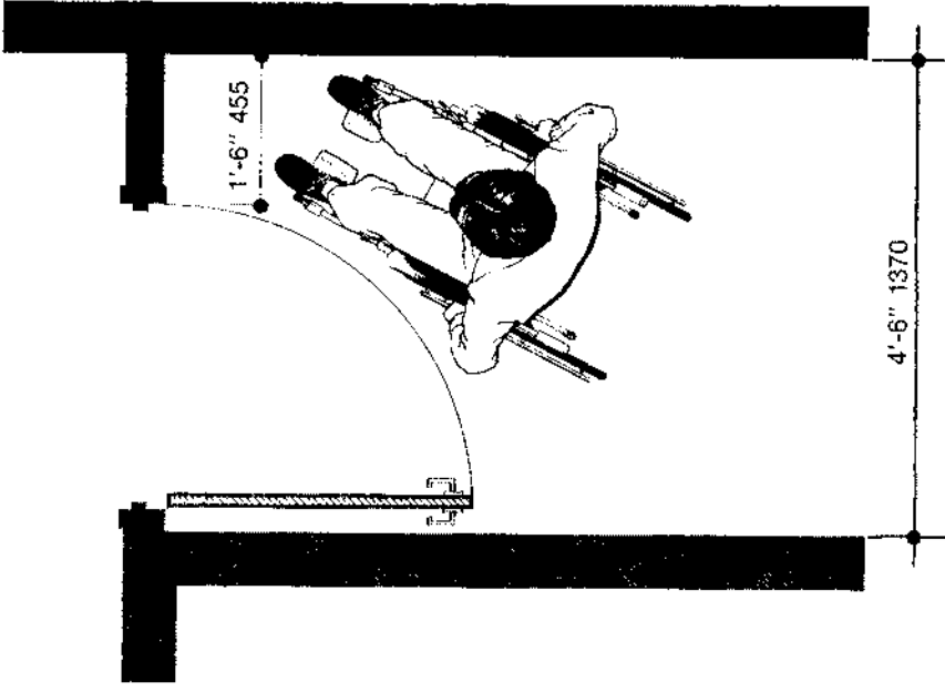
Figure 2.3.2 D Minimum dimension of corridor width with door opening into the corridor.
