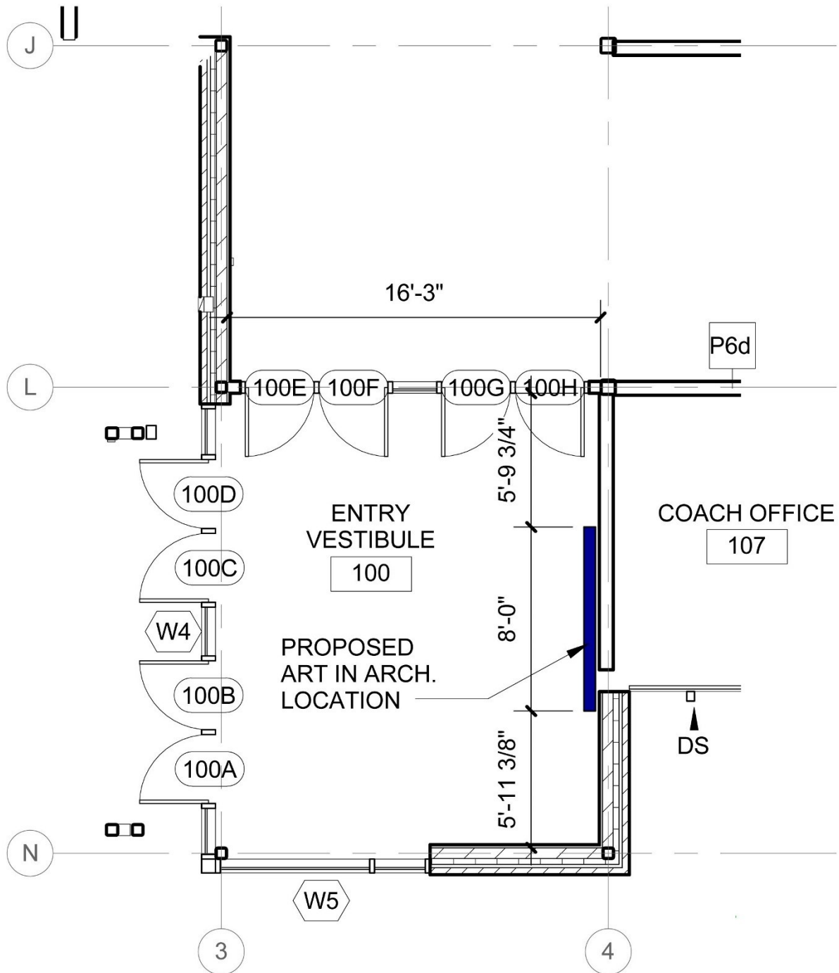
Entry Vestibule-Artwork Location, Plan View
