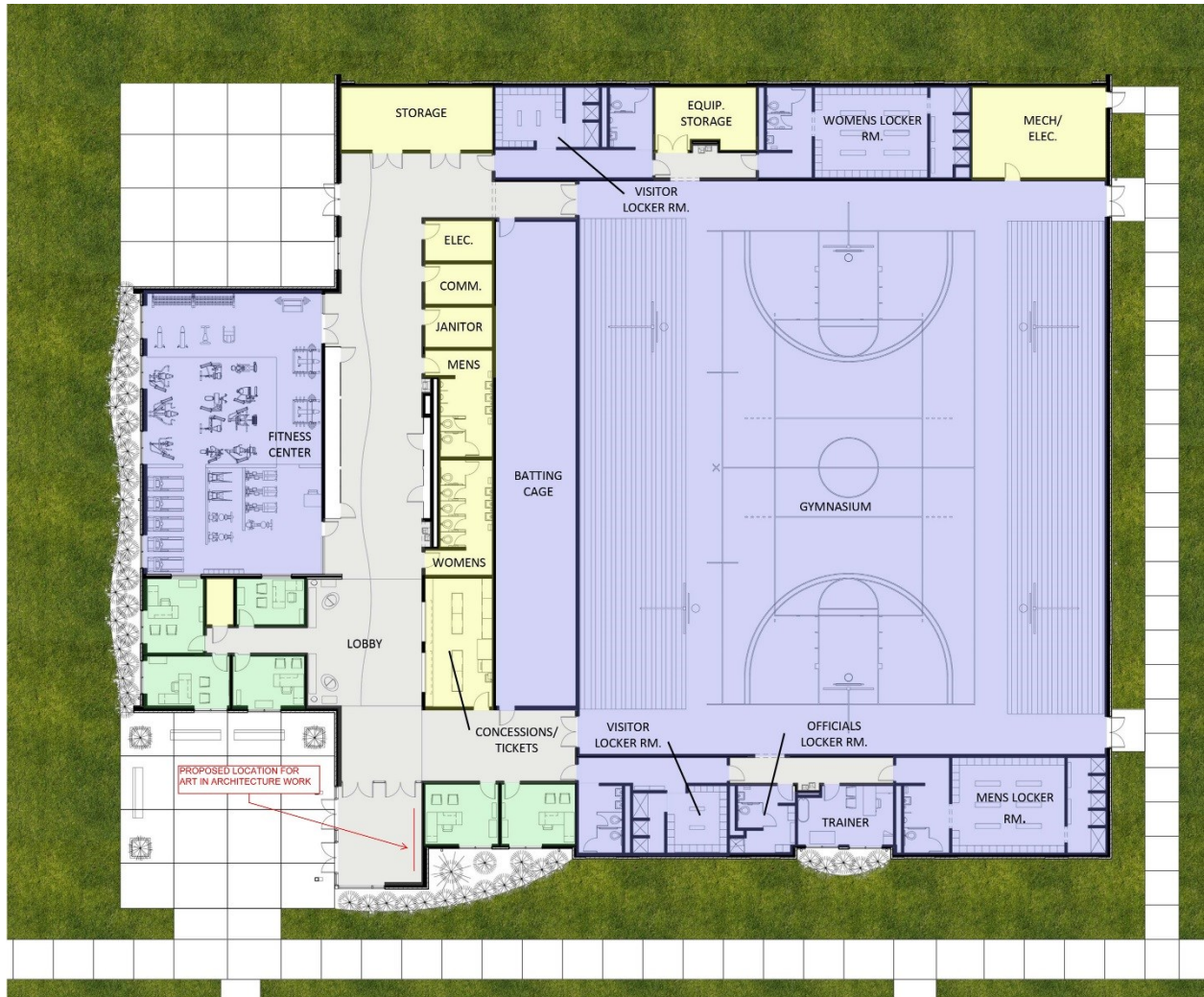
Floor Plan with Entry Vestibule Artwork Location
