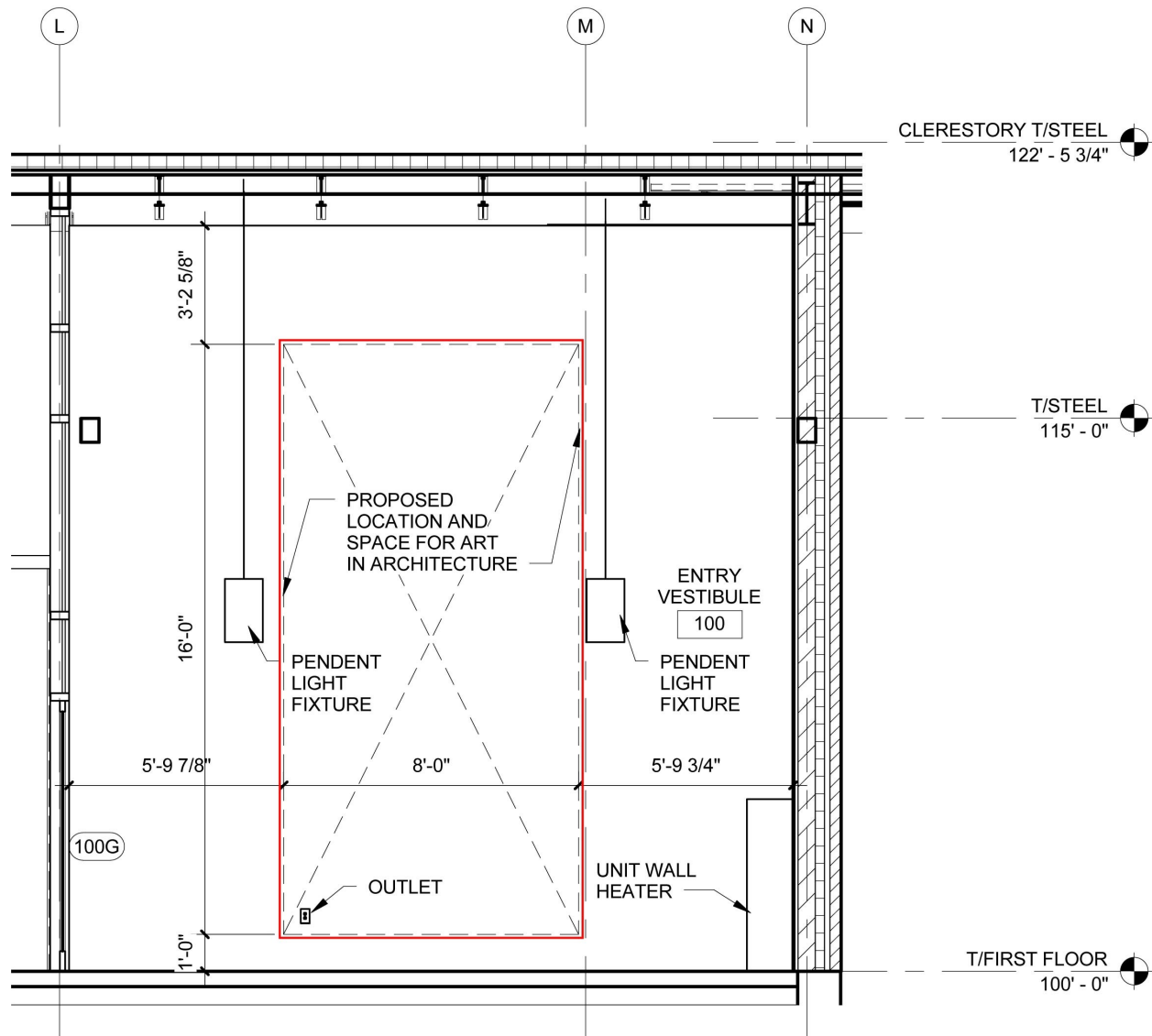
Entry Vestibule—Artwork Location, Elevation
